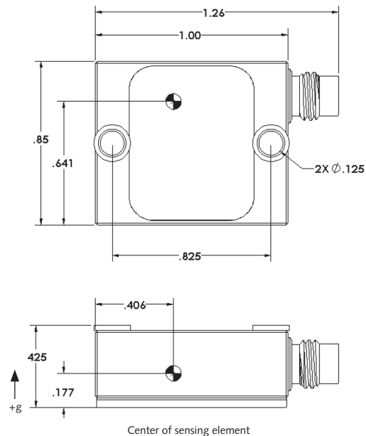
Outline drawing for Type 8316A...TA (units: mm [in])
