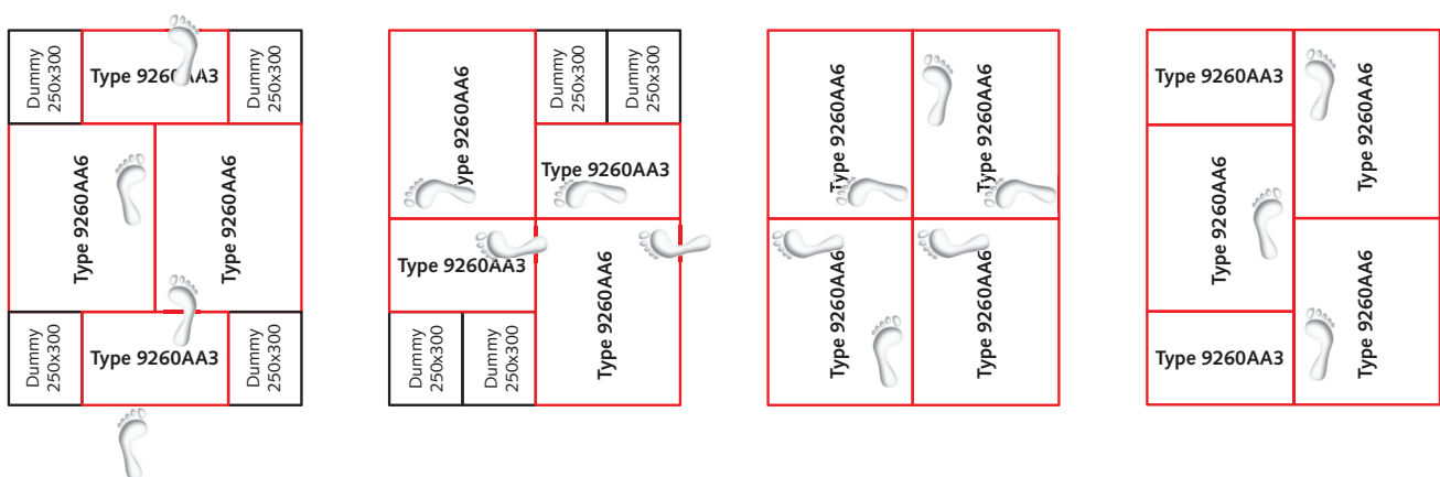
Fig. 1: Mounting examples for mounting frame Type 9428A1 with variable configuration of force plates
