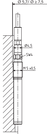
Fig. 2: Direct mounting
