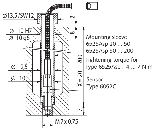
Fig. 3: Using the mounting sleeve
